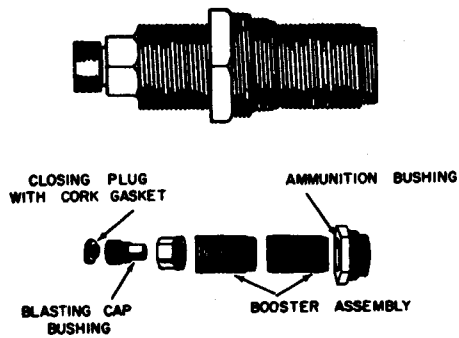
Figure 15 M10 Universal Explosive Destructor
